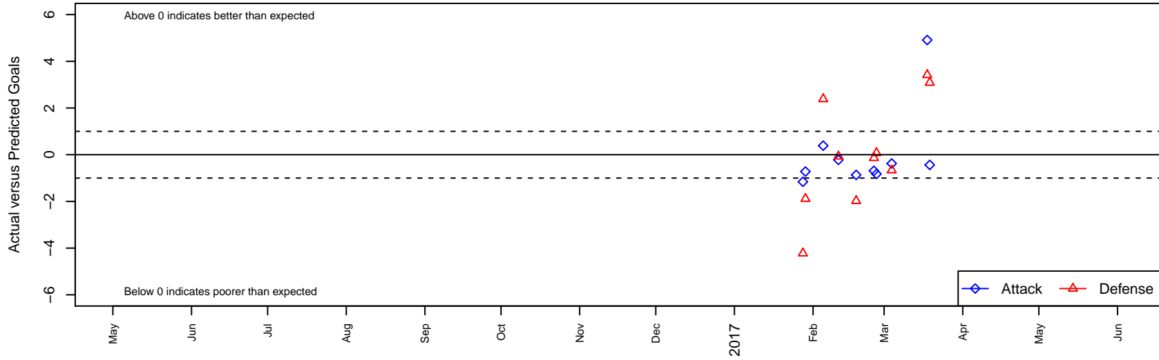
BSC Portland Grey B01 Dots are actual minus expected GF (blue circles) and GA (red triangles). Blue line is smoothed change in attack strength. Red is smoothed change in defense strength.
